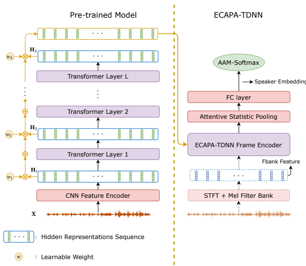
Fig. 1. Leverage Representations from Pre-trained Model
